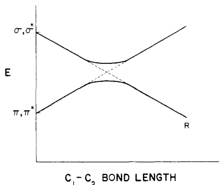
Figure 1. Correlation diagram for photochemical cyclopropane ring opening of arylcyclopropanes.
